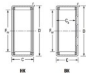
Metric parts with cage assembly
