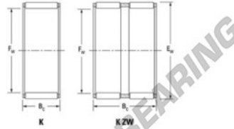
Boundary dimensions
